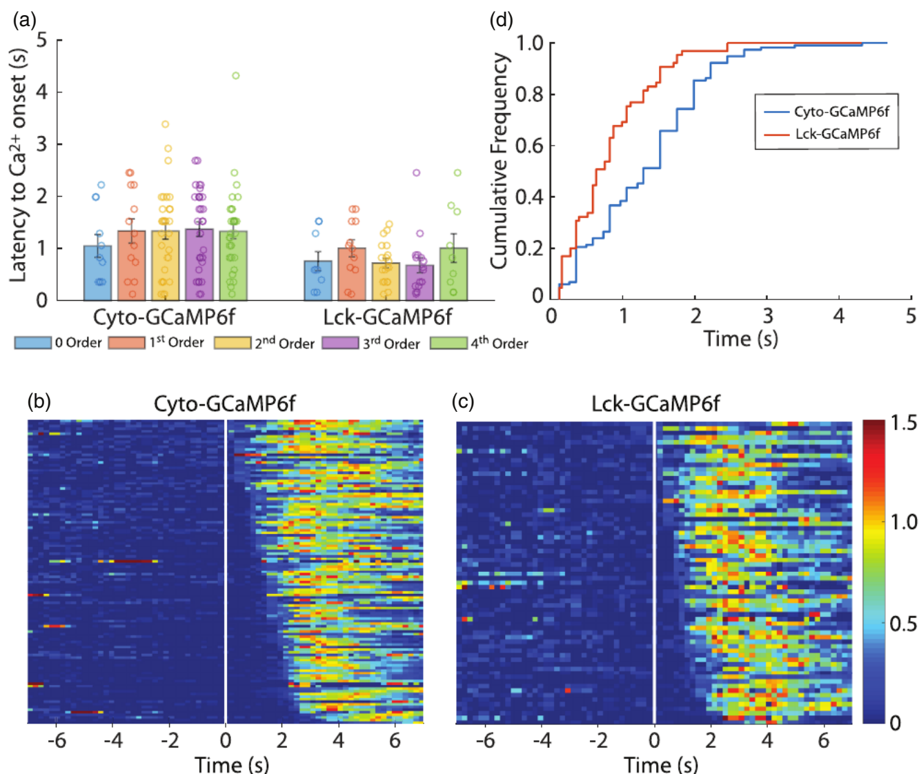
FIGURE 7 Latency to the onset of \text{Ca}^{2+} increase in astrocyte endfeet contacting vessels of different orders from WT mice trials without running. (a) Summary of latencies for each vessel order of mice expressing either Cyto-GCaMP6f (left, n = 11, 13, 30, 31, 32 for 0, 1st, 2nd, 3rd, 4th orders, respectively) or Lck-GCaMP6f (right, n = 9, 12, 19, 16, 9 for 0, 1st, 2nd, 3rd, 4th orders, respectively). Faster onset latencies were seen in Lck-GCaMP6f trials compared to Cyto-GCaMP6f. Mean \pm SEM plus individual vessels are shown. Two sample t-test between onset latency from combined orders of Cyto-GCaMP6f vs Lck-GCaMP6f, p = 9.0 \times 10^{-6} . (b & c) Heat maps showing \text{Ca}^{2+} responses from astrocyte endfeet contacting individual vessels. Records are sorted by latency. \text{Ca}^{2+} signals measured with Cyto-GCaMP6f (b, n = 117 ) and Lck-GCaMP6f (c, n = 65 ) are shown. \Delta F/F for each vessel was normalized to its peak \Delta F/F value. Trials where baseline variation exceeding 30% of peak \Delta F/F in the 2 s prior to the stimulus were excluded. Times are relative to stimulus onset (white vertical lines). (d) Cumulative plots of the onset latencies of astrocyte \text{Ca}^{2+} responses measured with Cyto-GCaMP6f (blue, n = 117 ) and Lck-GCaMP6f (orange, n = 65 ). A greater proportion of fast \text{Ca}^{2+} responses were recorded with Lck-GCaMP6f. Two sample Kolmogorov–Smirnov test, p = 1.25 \times 10^{-4}
