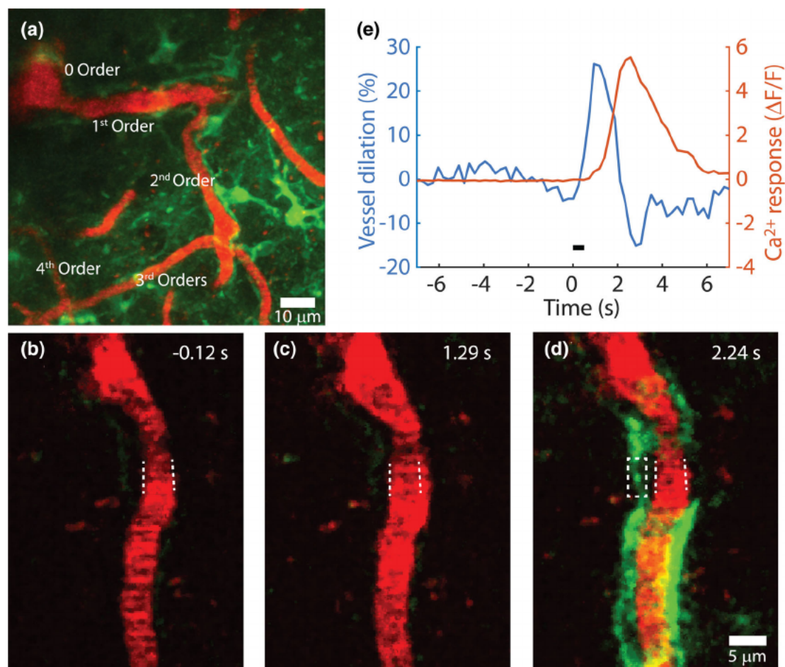
FIGURE 1 Measurement of vessel dilation and astrocyte endfoot Ca 2+ responses. (a) Maximum projection of a Z stack of 2P images showing 0 through 4th order blood vessels in the barrel cortex of the mouse. Vessels are labeled with Texas-red (red) and astrocytes express Cyto-GCaMP6f (green). (b to d) 2P images from a time series showing dilation of a WT 4th order capillary and Ca 2+ increases in adjacent endfeet. The hashed lines around the capillary indicate the width of the vessel before stimulation. The time of acquisition, relative to the onset of whisker stimulation, is indicated in each panel. (b) before stimulation. (c) near the peak of vessel dilation. (d) near the peak of the astrocyte Ca 2+ increase. The boxed area illustrates the ROI used to measure the endfoot Ca 2+ increase. (e) Traces showing capillary dilation (blue) and astrocyte Ca 2+ increases (orange) in the trial shown in panels b to d. The traces are an average of 9 no movement trials from the vessel. The black bar indicates the time course of the whisker stimulus
