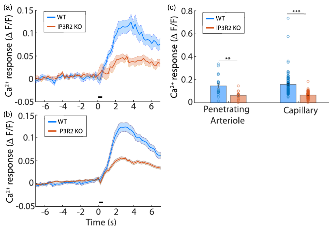
FIGURE 5 Astrocyte process \text{Ca}^{2+} responses near 0 order penetrating arterioles and 1st through 4th order capillaries. (a) Evoked \text{Ca}^{2+} responses in astrocyte processes near 0 order penetrating arterioles measured with Lck-GCaMP6f in WT ( n = 21 ) and IP3R2 KO ( n = 15 ) animals. Mean \pm SEM of all Lck-GCaMP6f 0 order trials. (b) Evoked \text{Ca}^{2+} responses in astrocyte processes near 1st through 4th order capillaries measured with Lck-GCaMP6f in WT ( n = 95 ) and IP3R2 KO animals ( n = 108 ). Mean \pm SEM of all Lck-GCaMP6f 1st through 4th order capillary trials. (c) Summary of results, showing the decrease of evoked \text{Ca}^{2+} responses in astrocyte processes near dilating blood vessels. Two sample t-tests of WT and IP3R2 KO animal. ** p < 0.01 , *** p < 0.001
