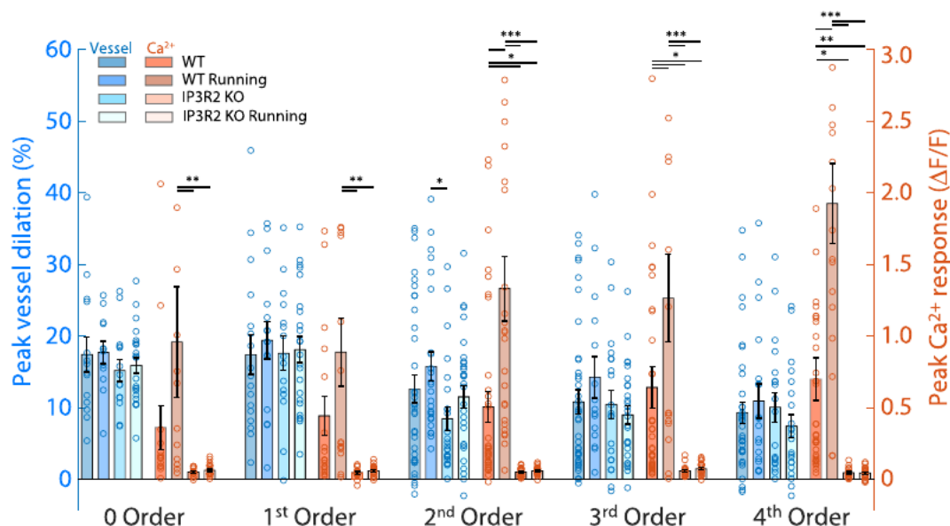
FIGURE 3 Summary of vessel dilation and astrocyte endfoot \text{Ca}^{2+} responses for all order vessels. Peak vessel dilation (blue) and astrocyte \text{Ca}^{2+} increases (orange) for WT, WT running, IP3R2 KO, and IP3R2 KO running groups for all order vessels are shown as mean \pm SEM plus individual vessel values. Astrocyte \text{Ca}^{2+} increases displayed are from Cyto-GCaMP6f recordings. Astrocyte \text{Ca}^{2+} increases in WT running trials were significantly larger compared to no running WT trials. Compared to WT and WT running, astrocyte \text{Ca}^{2+} increases in IP3R2 KO groups were significantly decreased. However, across all order vessels, vessel dilations remained largely unchanged despite the increased or decreased astrocyte \text{Ca}^{2+} signaling. Two-way ANOVA between genotype and movement conditions for each vessel order, Tukey–Kramer post hoc. Between the different orders, both 0 and 1st order vessels ( n = 63 and 70 , respectively) dilated more than 2nd, 3rd, and 4th order vessels ( n = 114 , 100 , and 94 , respectively). One-way ANOVA, Tukey–Kramer post-hoc test, p < 0.05 . * p < 0.05 , ** p < 0.01 , *** p < 0.001 . Tables 1 to 4 contain a summary of the data displayed, including the n 's for each category
