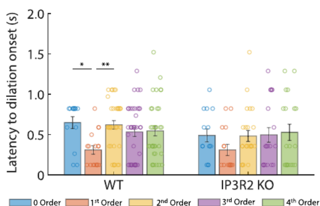
FIGURE 6 Latency to the onset of vessel dilation for all order vessels from WT and IP3R2 KO mice trials without running. 1st order capillaries had a faster dilation onset compared to 0 order penetrating arterioles and 2nd order capillaries. One-way ANOVA between the orders of each genotype, Tukey-Kramer post hoc. * p < 0.05 , ** p < 0.01 . Mean \pm SEM plus individual vessels are shown. Tables 1 and 2 Contain a summary of the data displayed, including the n's for each category
