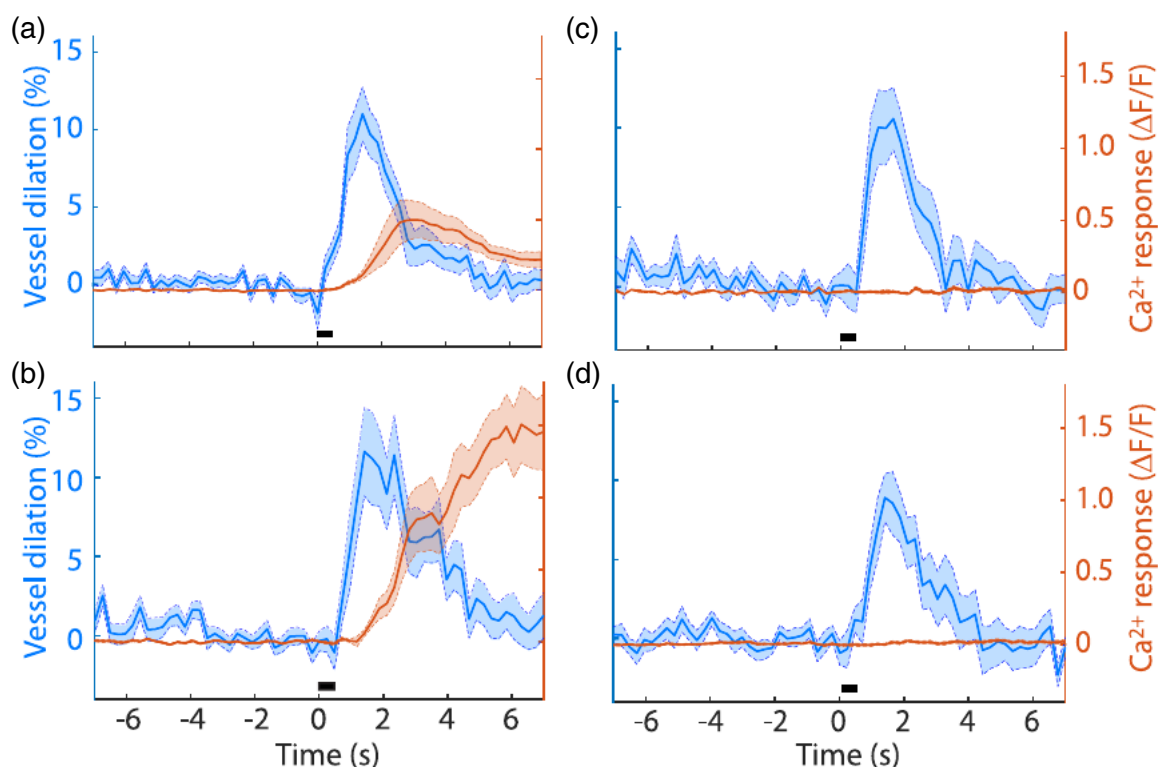
FIGURE 2 Average responses of 4th order capillaries and adjacent astrocyte endfeet to whisker stimulation. Mean \pm SEM vessel dilations (blue) and astrocyte \text{Ca}^{2+} increases (orange) are shown. Black bars indicate the time course of the whisker stimulus. (a) Trials where WT mice did not run. N = 35 vessels. (b) Trials where the stimulus evoked running in WT mice. Running elicited increased astrocyte \text{Ca}^{2+} signaling compared to trials where mice did not run. N = 18 vessels. (c) Trials of IP3R2 KO mice where the animal did not run. The evoked astrocyte \text{Ca}^{2+} response is largely eliminated compared to WT trials. N = 19 vessels. (d) Trials of IP3R2 KO mice where the stimulus evoked running. N = 22 . Despite the widely varying \text{Ca}^{2+} responses under the four conditions, vessel dilation remained largely unchanged
