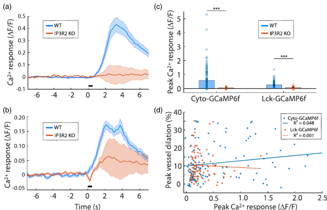
FIGURE 4 Astrocyte endfoot \text{Ca}^{2+} responses and resulting vessel dilations of 1st through 4th order capillaries. (a) Evoked \text{Ca}^{2+} responses in astrocyte endfeet measured with Cyto-GCaMP6f in WT ( n = 129 ) and IP3R2 KO ( n = 78 ) animals. Mean \pm SEM of all 1st through 4th order capillary trials. (b) Evoked \text{Ca}^{2+} responses in astrocyte endfeet measured with Lck-GCaMP6f in WT ( n = 96 ) and IP3R2 KO ( n = 110 ) animals. Mean \pm SEM of all 1st through 4th order capillary trials. (c) Summary of results, showing the decrease of evoked \text{Ca}^{2+} responses in IP3R2 KO animals measured with both Cyto- and Lck-GCaMP6f \text{Ca}^{2+} indicators. Two sample t test of WT and IP3R2 KO capillary endfeet peak \text{Ca}^{2+} responses, ***p < 0.001 . (d) Scatterplot showing relation between the evoked astrocyte \text{Ca}^{2+} increase and the corresponding capillary dilation for individual capillaries for all 1st through 4th order capillaries. Lines indicate least-squares fit for trials using the Cyto (blue, n = 129 ) and Lck (orange, n = 96 ) \text{Ca}^{2+} indicators. The R^2 coefficient of determination values are indicated
